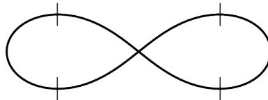
Figure 1: Sketch of the lemniscate from Gauss’s notebook, from [Gauss, 1876]
